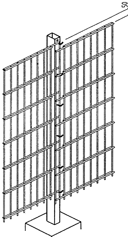
② Left-hand mesh panel hung normally, right-hand panel 50mm lower.
