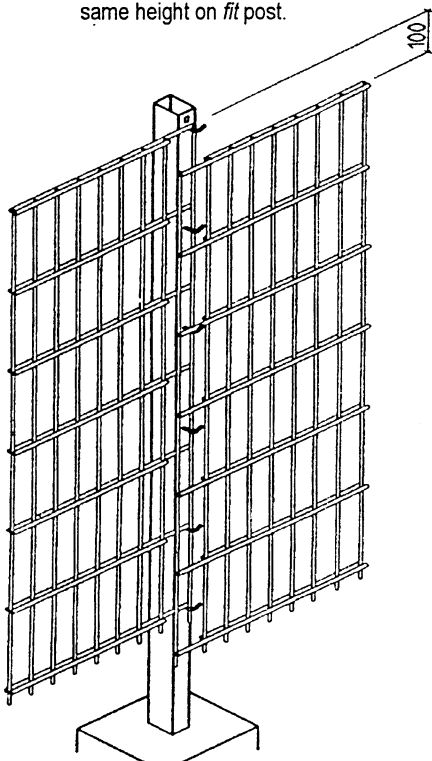
③ Left-hand mesh panel hung normally, right-hand mesh panel 100mm lower.
